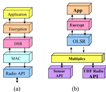
Figure 2: Generic Communication Stack
